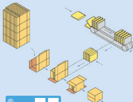
operating principle of olibag 210 with olimat 1 : with wrap-around cases
